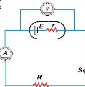
Fig. 9.27: The terminal potential difference V of a cell is E - Ir .
