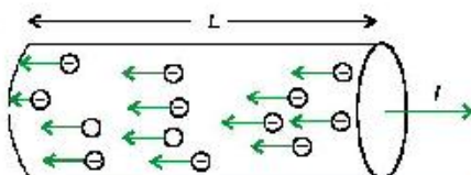
Fig. 9.22: Negative charge carriers
