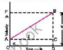
Fig. 2.8: Velocity-Time Graph
