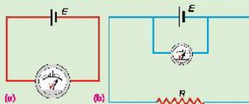
Fig. 9.27: The terminal potential difference V of a cell is E - Ir .
