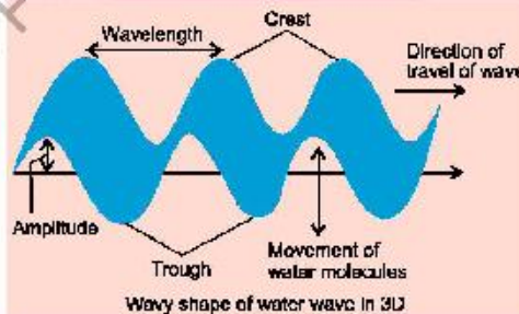
Fig. 7.2: Graphical description of a wave
