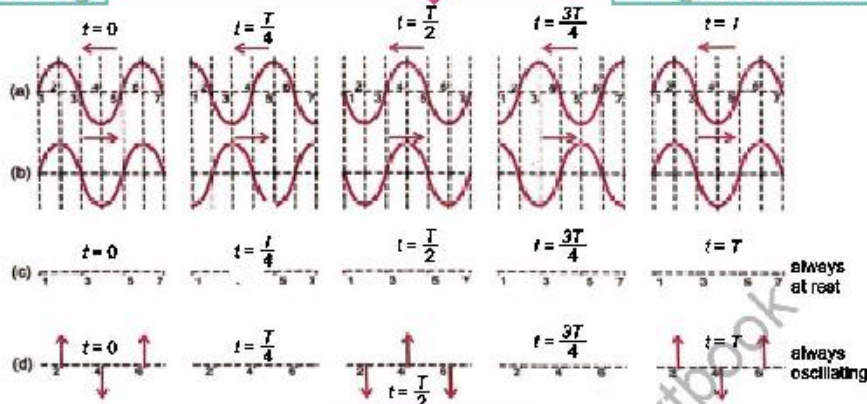
Fig. 7.6: Stationary waves
