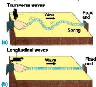
Fig. 7.3: Main types of waves
