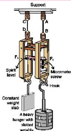
Fig. 5.4: Searle's apparatus
