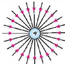
Fig 9.7: The electric field lines are directed radially inward towards a negative point charge -q .
