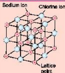
NaCl crystal lattice
