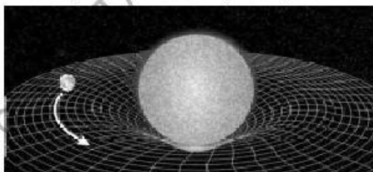
Spacetime curve shown by two satellites
