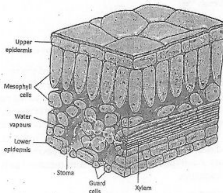
FIGURE 9.3: Events of transpiration
