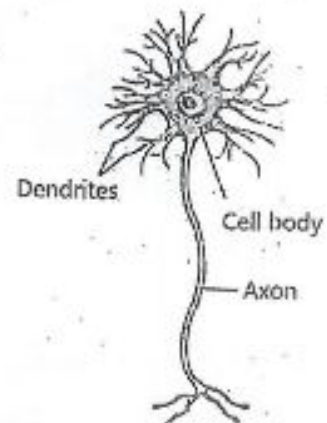
FIGURE 3.19: Neuron
