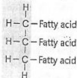
Fats and oils General structure
