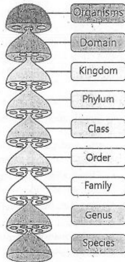
FIGURE 2.1: Taxonomic ranks
