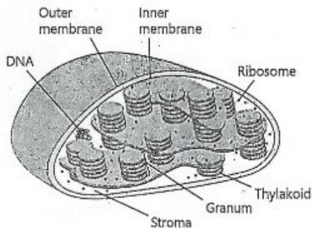
FIGURE 3.13: A Chloroplast
