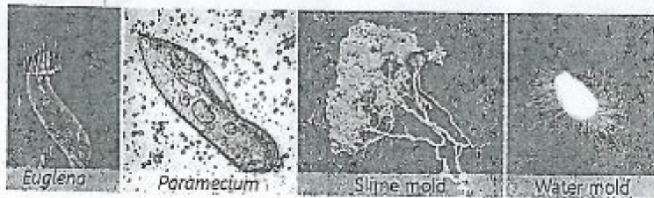
FIGURE 2.5: Common protists
