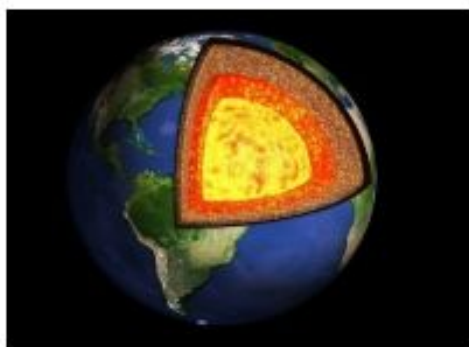
Internal structure of the Earth
