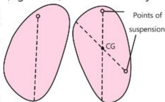
Fig. 4.15(a) Fig. 4.15(b) Irregular shaped plane lamina
