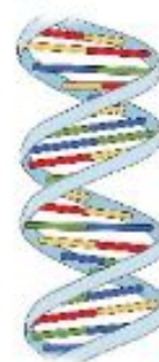
DNA Structure
