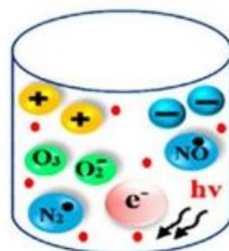
Fig. 7.3(a) Plasma
