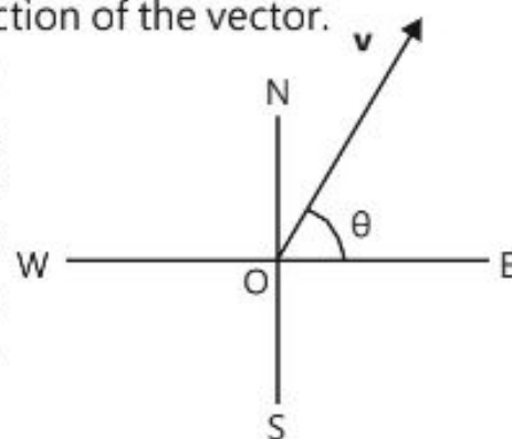
A vector v making an angle \theta towards north from east
